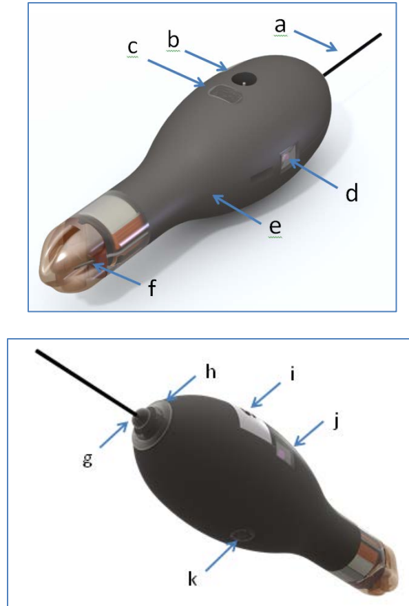
Figure 2 – sPAT tag showing: (a) Argos antenna, (b) temperature sensor, (c) communications port with plug, (d) light sensor (1 of 2), (e) float, (f) release pin, (g) LED light, (h) wet/dry sensor, (i) ground plate, (j) light sensor (2 of 2), and (k) pressure sensor
